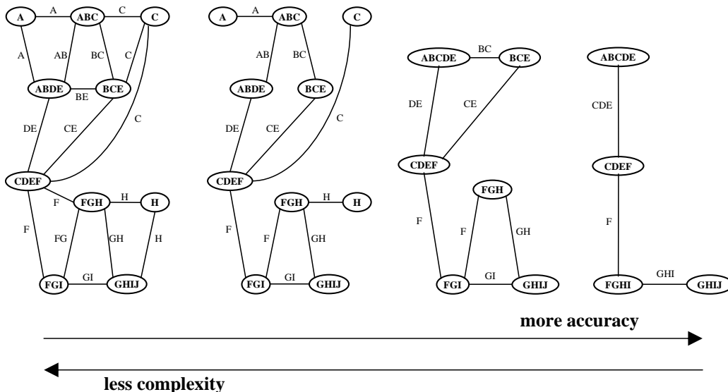
Figure 19: Join-graphs.
