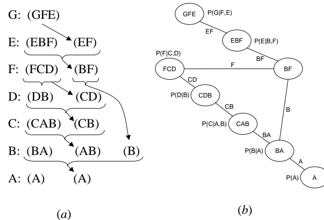
Figure 18: Join-graph decompositions.
